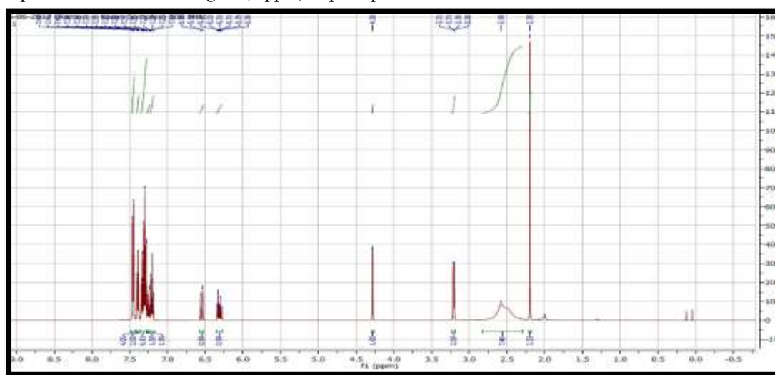
Figure 2 1 H NMR Spectrum of sample drug Cinnarizine HCL
