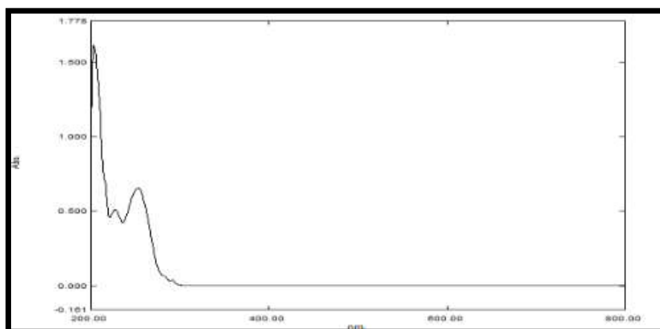
Figure 4 UV Spectroscopy of CNZ for Detection of \lambda_{\text{max}} in 0.1 N HCL
