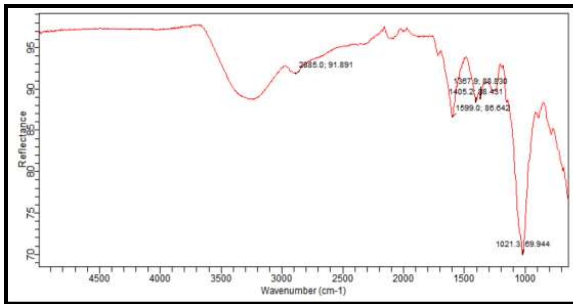
Figure 8 FTIR Spectrum of CNZ + XG
