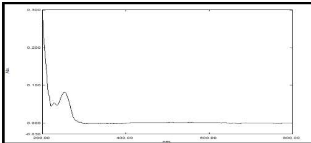
Figure 5 Calibration curve of CNZ with 0.1 N HCL
