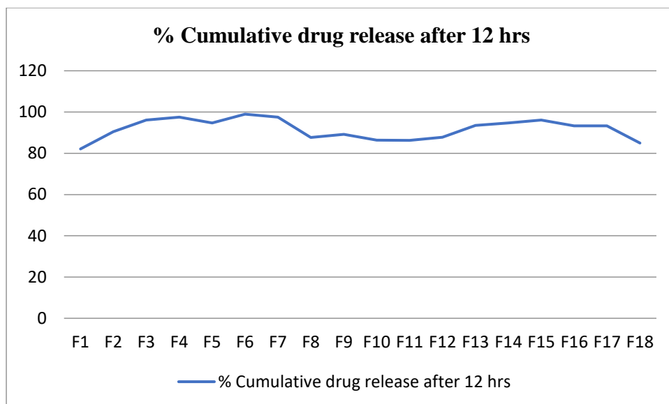
Figure 15 Cumulative Percentage drug release after 12 hours
