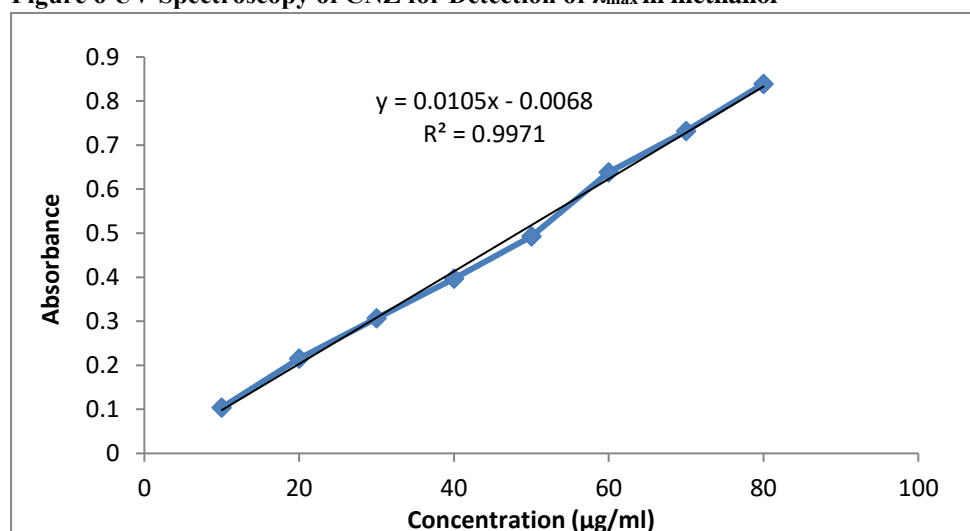
Figure 7 Calibration Curve of CNZ in methanol
