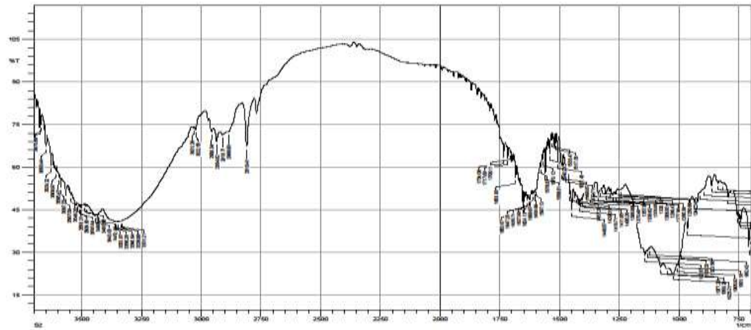
Figure 10 FTIR Spectrums of CNZ + CMC Sodium
