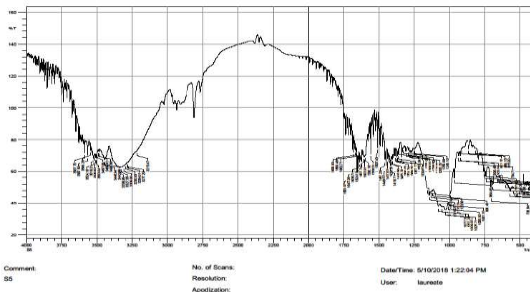
Figure 14 FTIR Spectrum of CNZ+ SA+ XG
