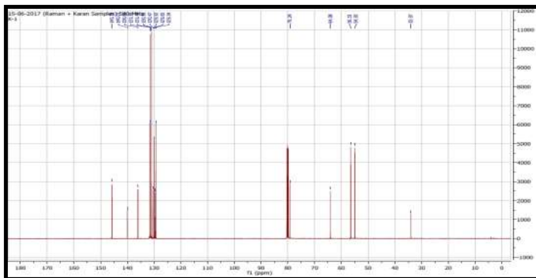
Figure 3 C^{13} NMR Spectrum of sample drug Cinnarizine HCL
