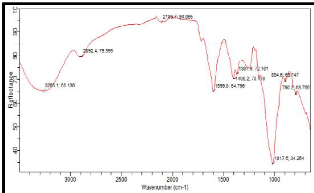
Figure 9 FTIR Spectrum of XA
