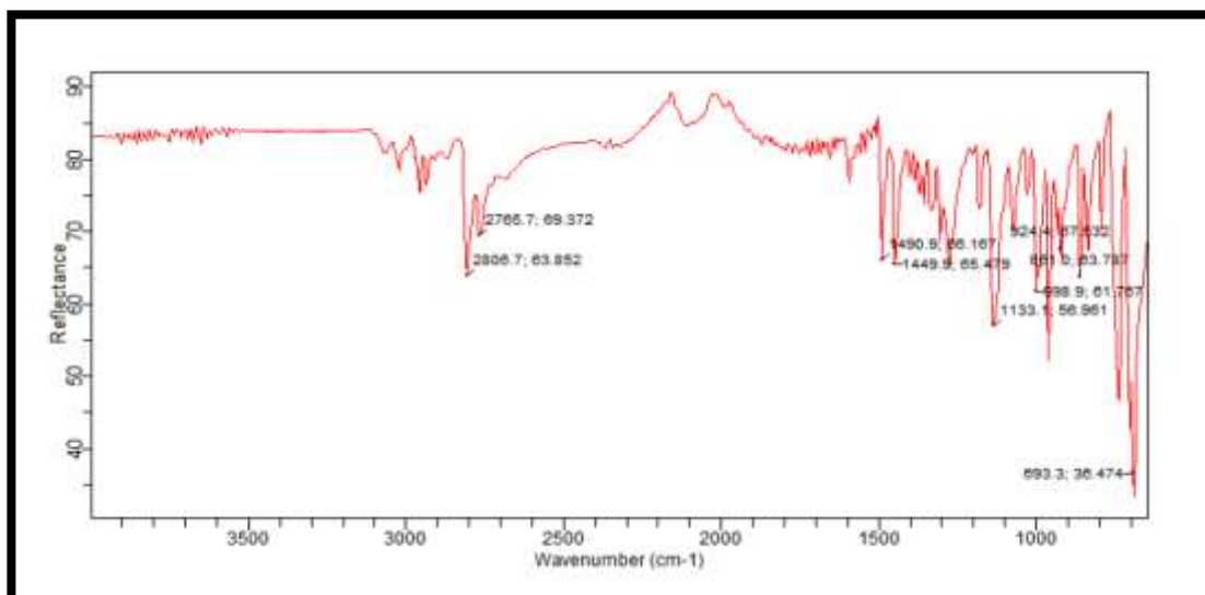
Figure 1 FTIR Spectrum of sample drug CNZ
