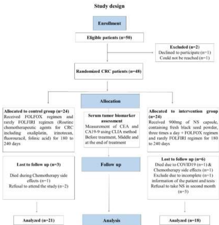
Figure 1. Study design.
