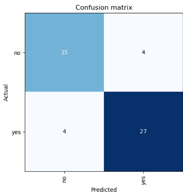
Figure 4: Confusion Matrix
