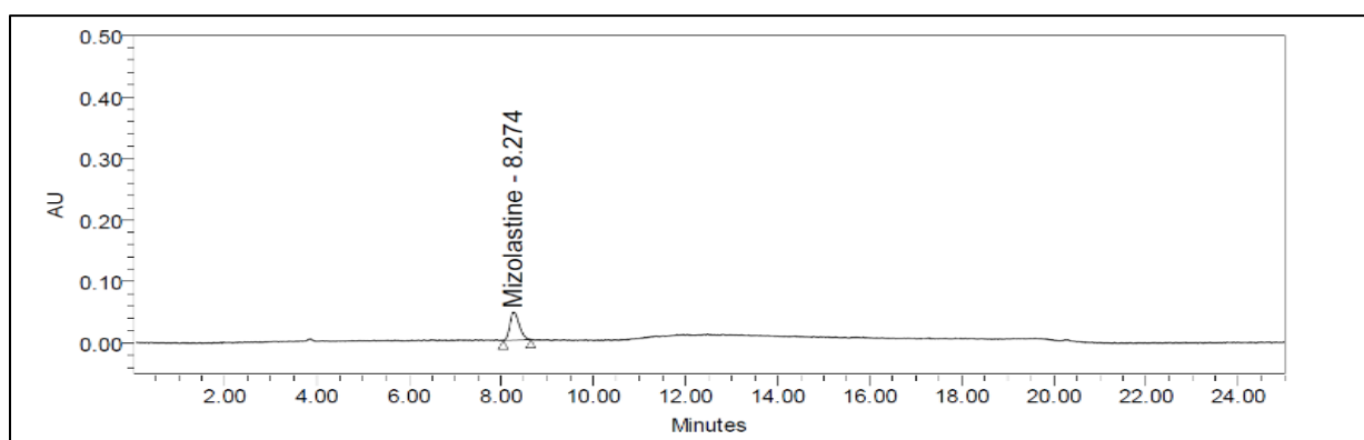
Fig. 3. Standard Chromatogram
