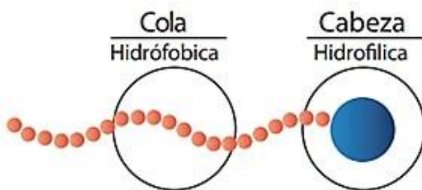
Figure 4. Surfactant Groups [10].
