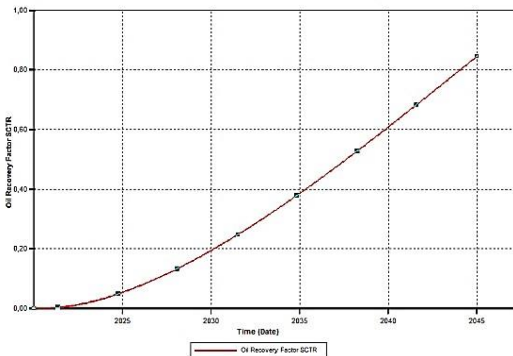
Figure 20. Recovery Factor - Surfactant Injection
