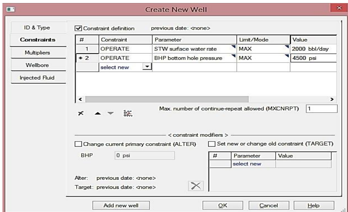
Figure 13. Injector Well
