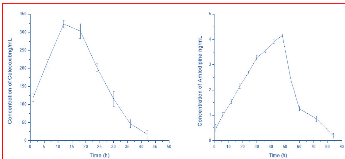
Figure 5: Mean plasma concentration- time profiles of Celecoxib and Amlodipine
