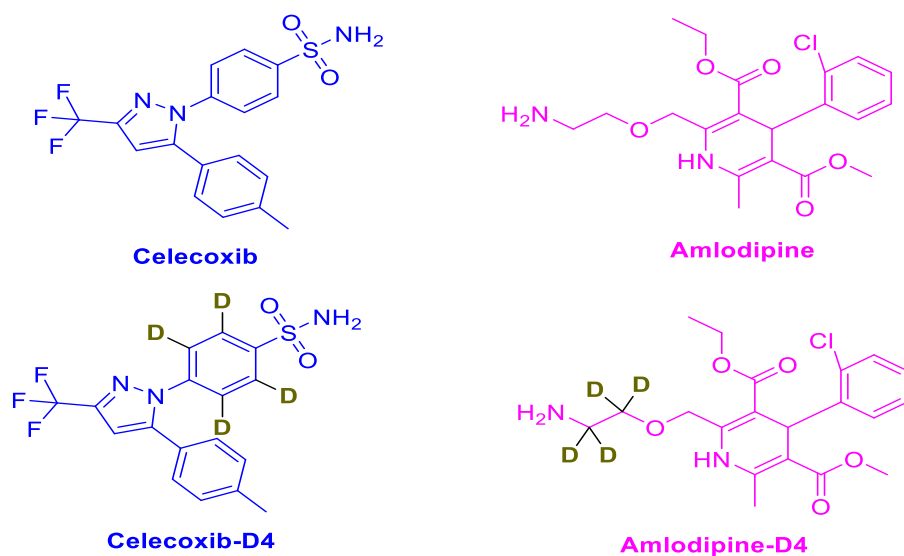
Figure 1: Chemical structure of Celecoxib, Amlodipine, and internal standards Celecoxib-D4 and Amlodipine-D4
