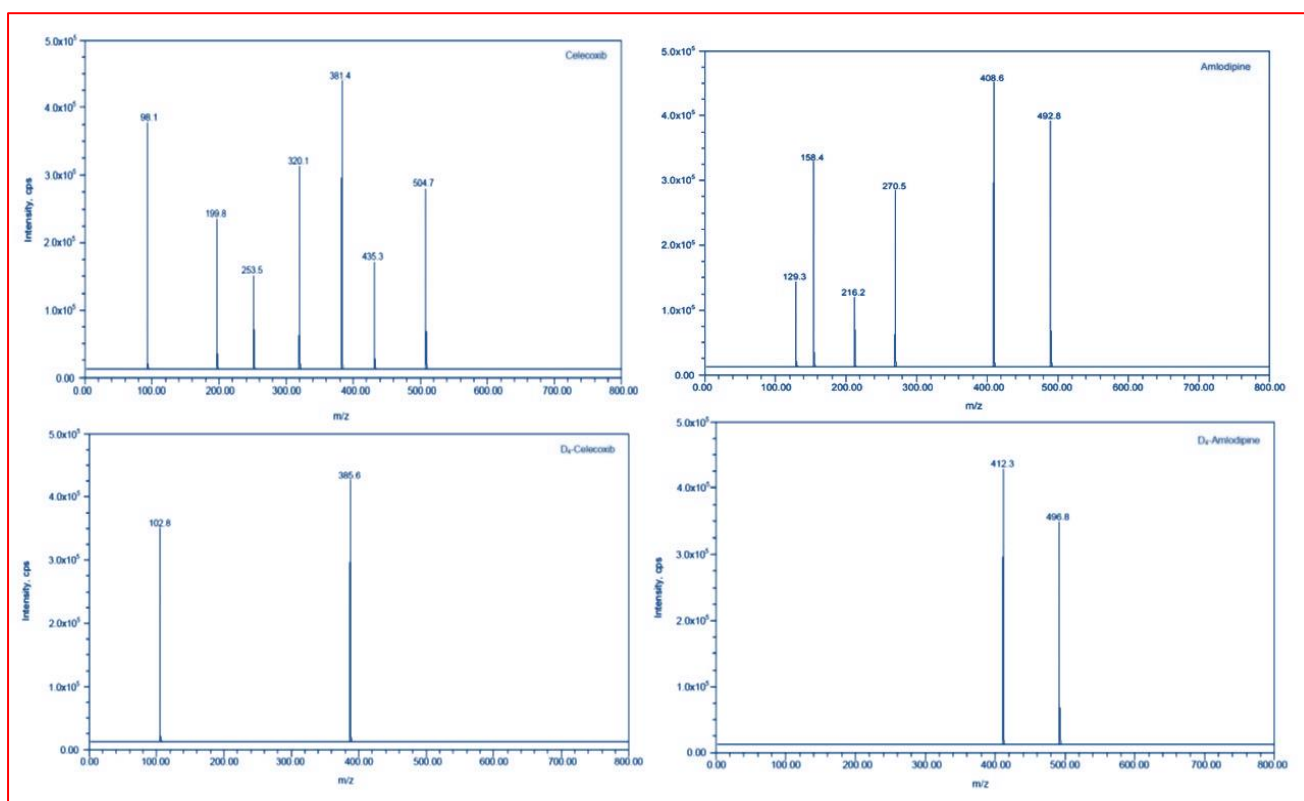
Figure 2: Product ion spectra of Celecoxib, Amlodipine, Celecoxib-D4 and Amlodipine-D4
