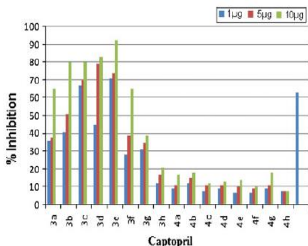
Fig. 2 ACE inhibition by tetrazoles 3a–3h and oxadiazoles 4a–4h
