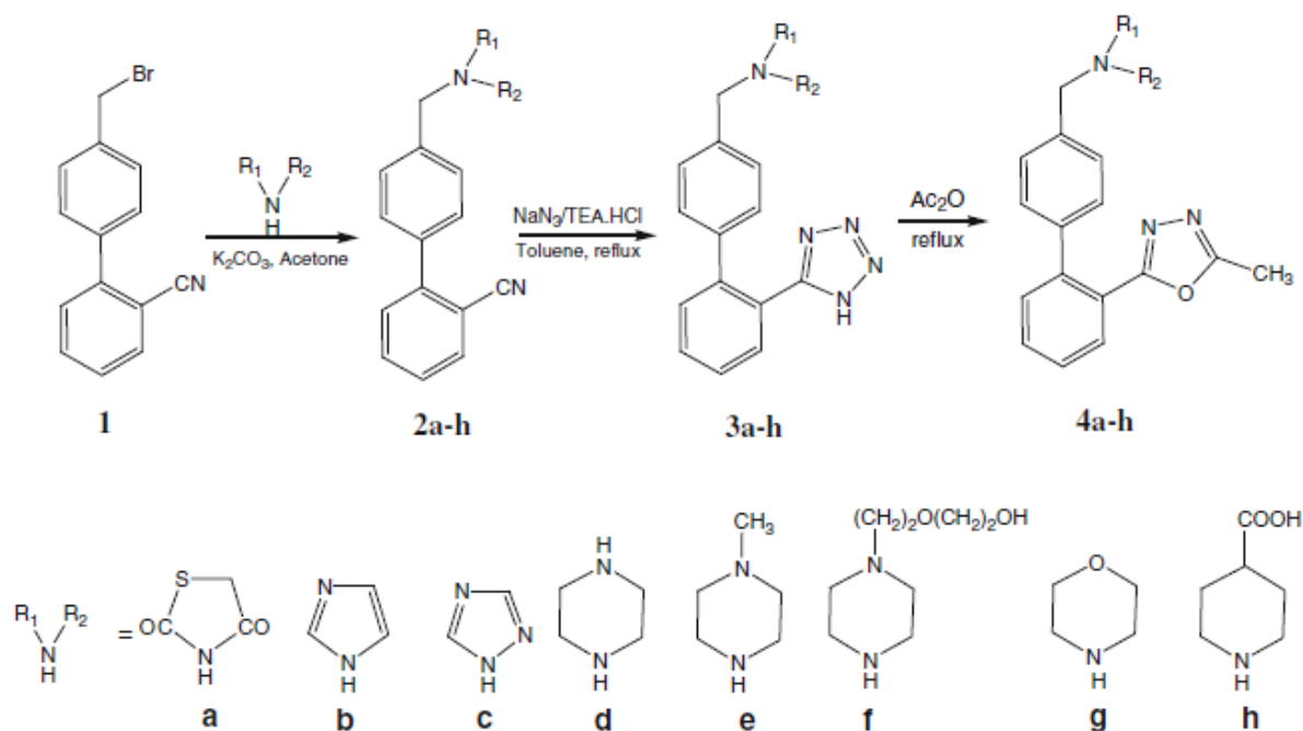
Scheme 1 Protocol for the synthesis of biphenyl derivatives
