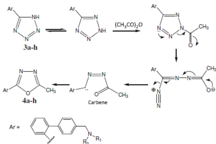
Scheme 2 Mechanism for ring transformation of tetrazole 3a–3h into oxadiazole 4a–4h
