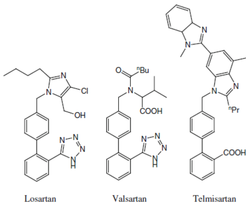
Fig. 1 Angiotensin receptor antagonists (Sartans)
