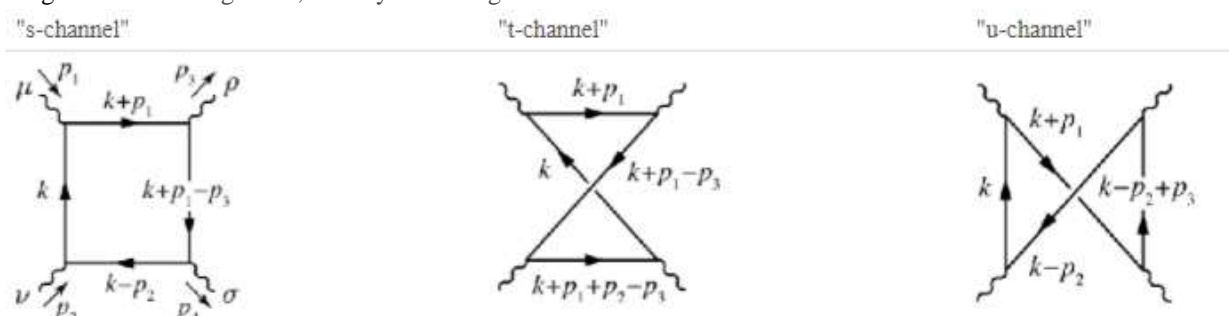
Figure 1: st-channel diagram for \gamma\gamma \rightarrow \gamma\gamma process
